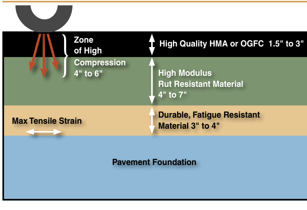
Figure 3. Perpetual Pavement Design Concept
